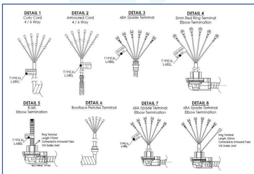
Complete termination details
