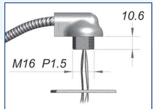
Elbow detail
