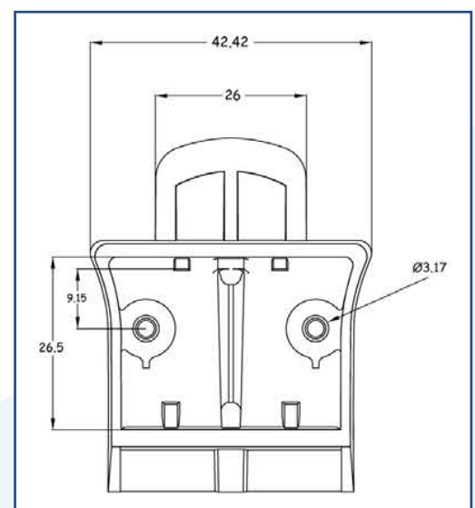
Hang-up hook detail
