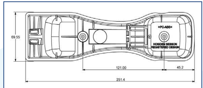
Cradle installation
